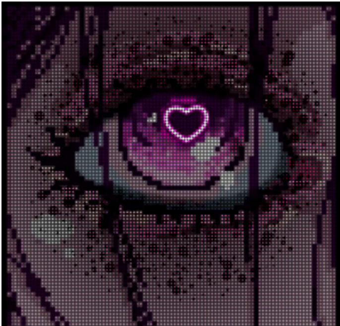
Original
