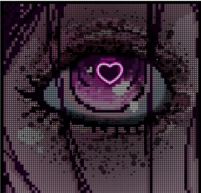
Sharpened
